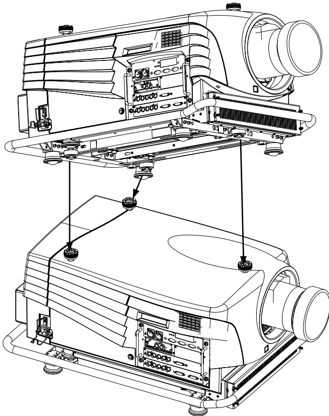
Image 3-22 Stacking two projectors
