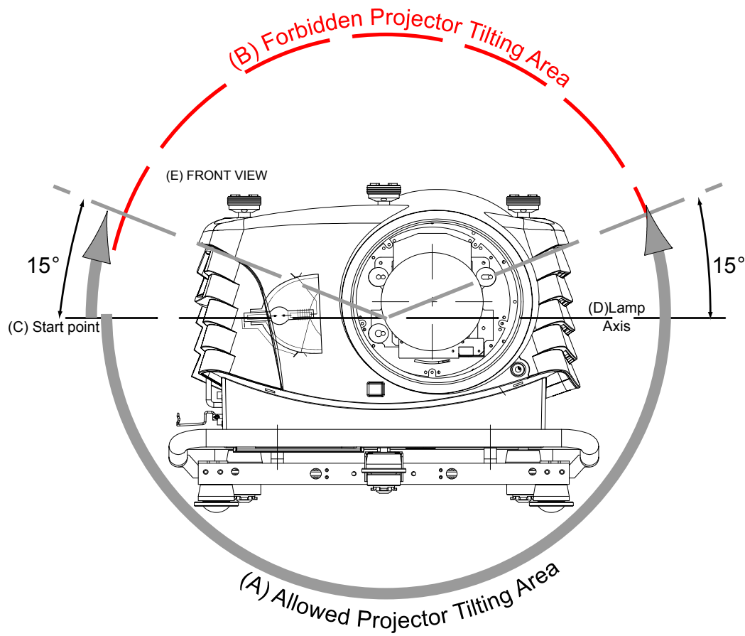
Image 3-7 Tilting diagram
