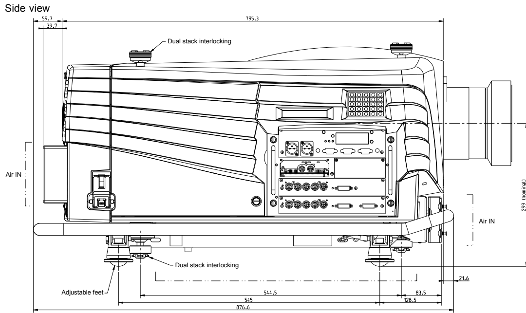
Image 2-3 Side view dimensions
