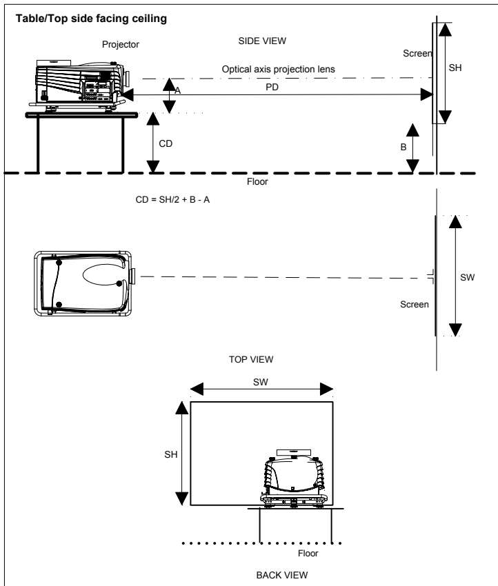
Image 3-2 Table mounted configuration
