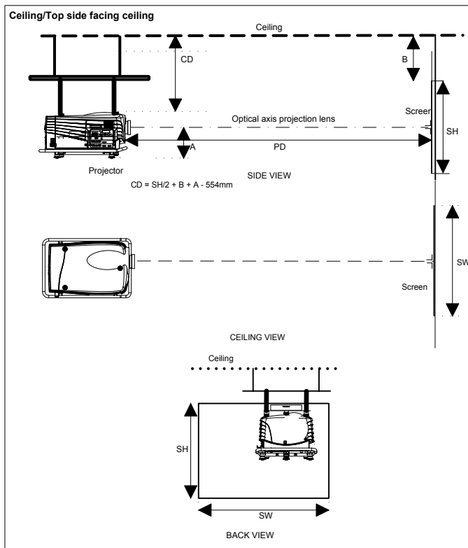
Image 3-5 Ceiling mounted projector
