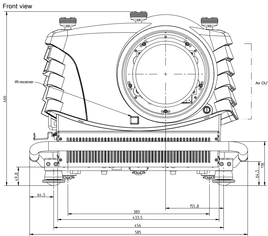
Image 2-2 Front view dimensions
