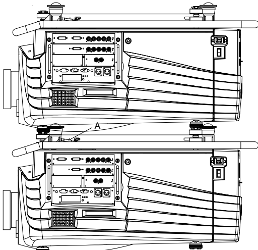
Image 3-24 Mounting the security chain
