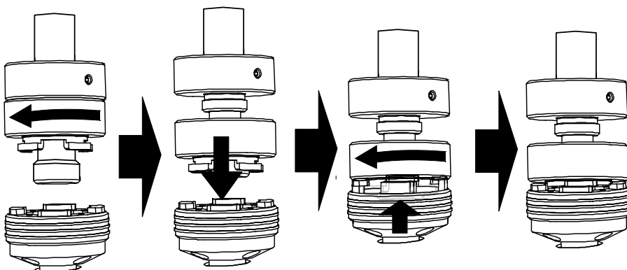
Image 3-23 Closing the rigging sockets
