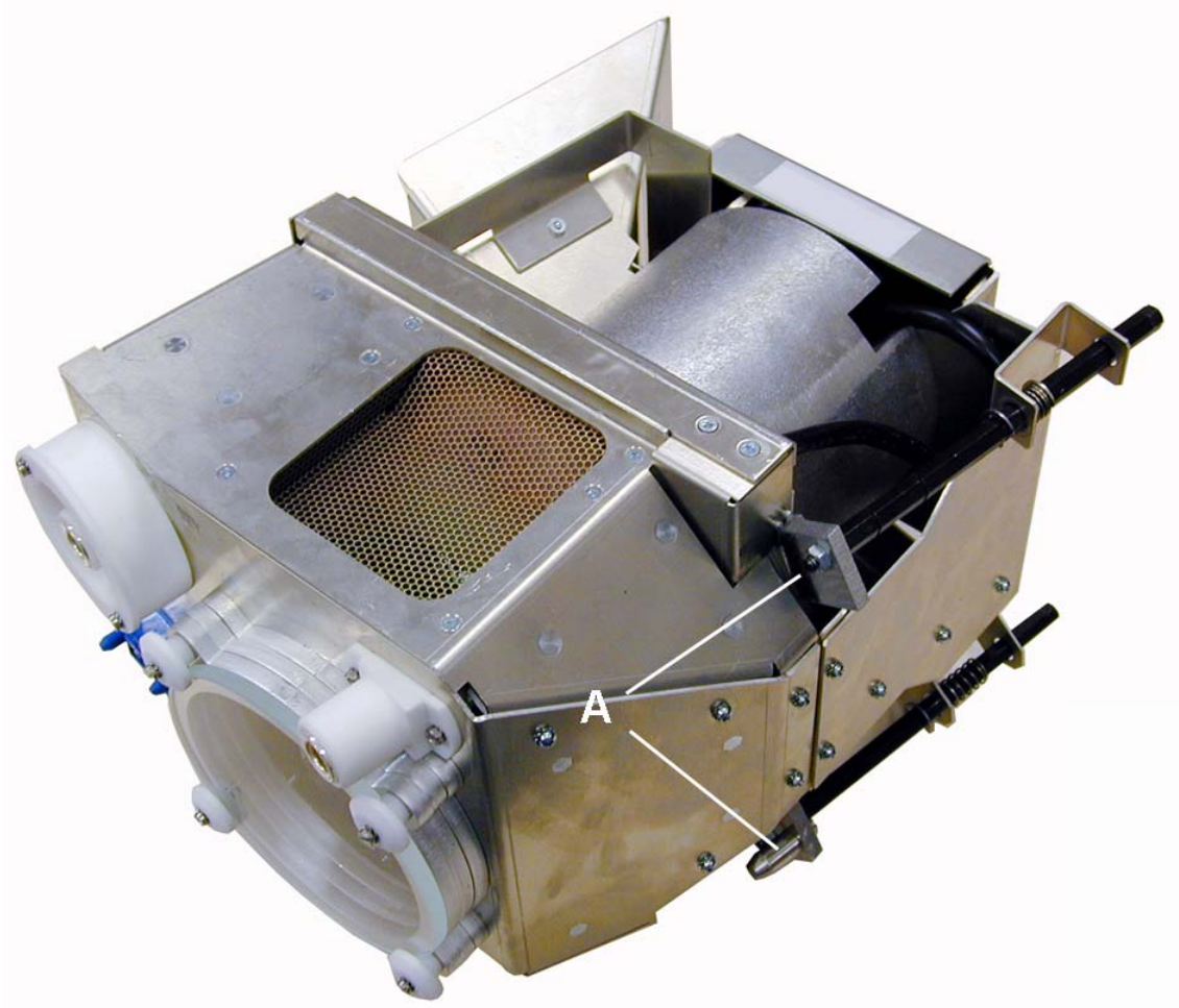
Image 3-10 Lamp unit, removing the lock nuts
