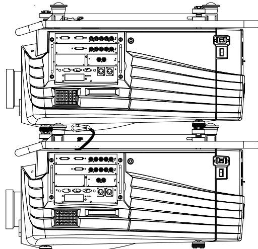
Image 3-25 Mounting the security hook
