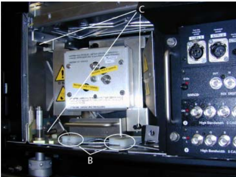
Image 3-12 Securing the lamp
