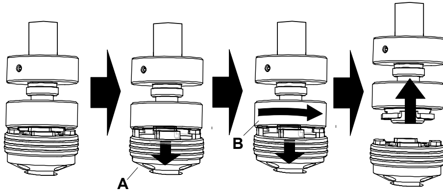
Image 3-27 Opening the rigging sockets
