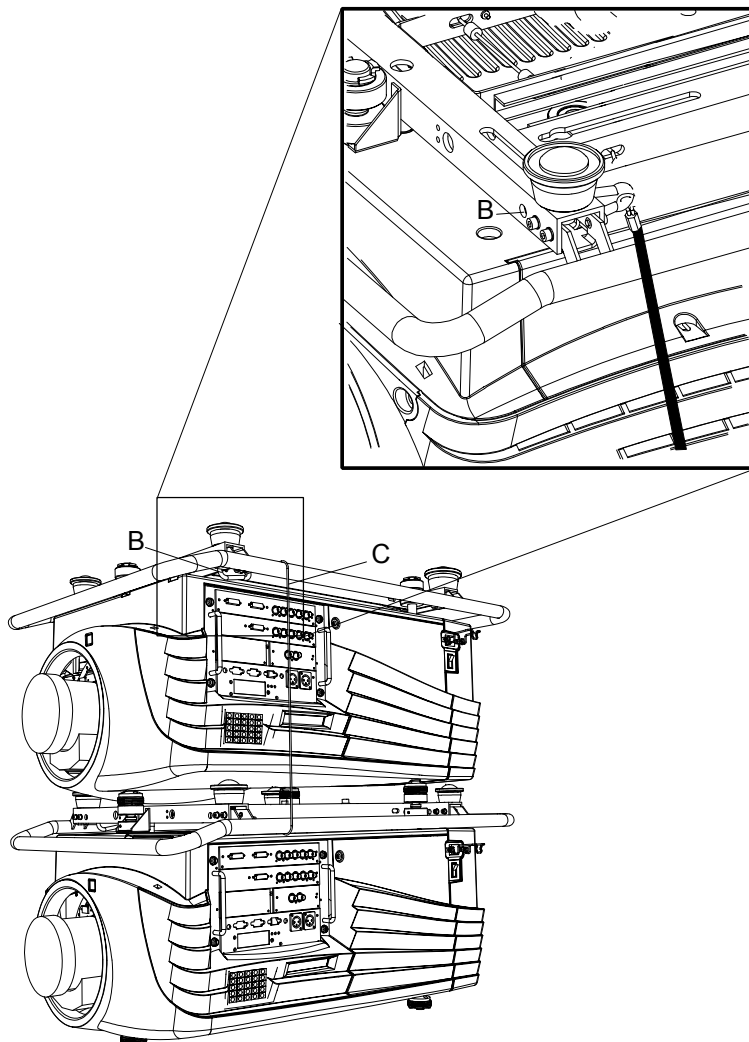
Image 3-26 Mounting the security hook (detail)
