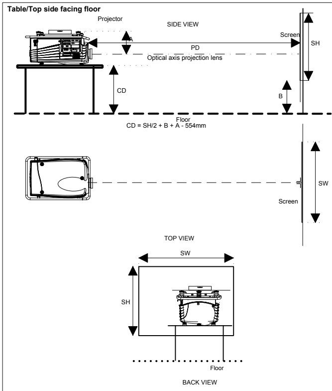
Image 3-3 Table mounted configuration up side down
